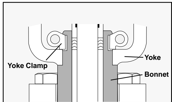
Figure 8: Yoke Clamp
